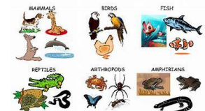
ANIMAL CLASSES
